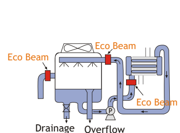
Cooling Tower Heat Exchanger
