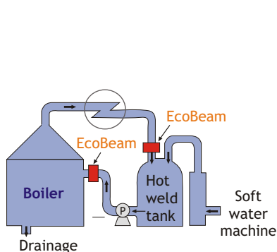
Boiler
