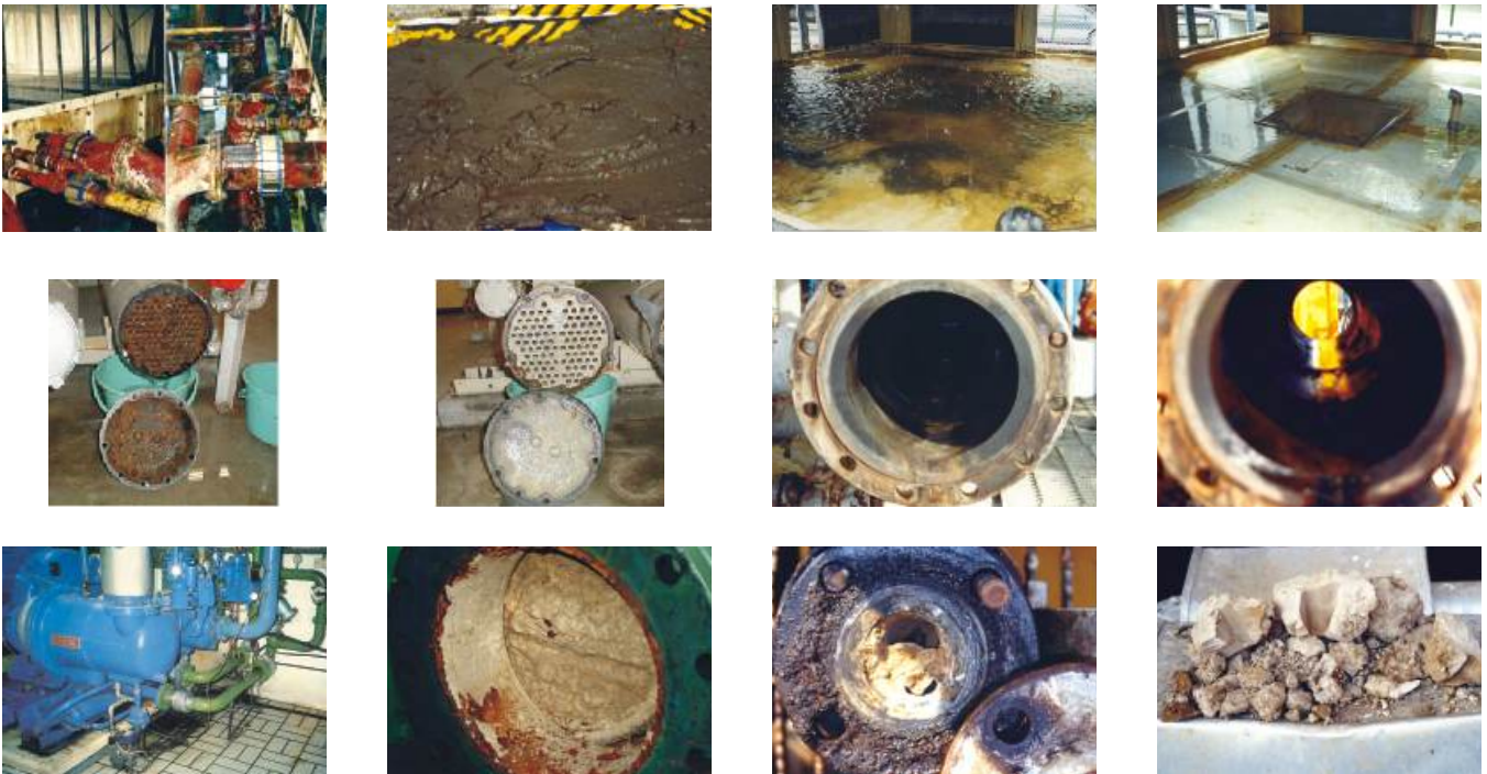
A Heat Exchanger/Cooling Tower System before and after installation of EcoBeam XL
